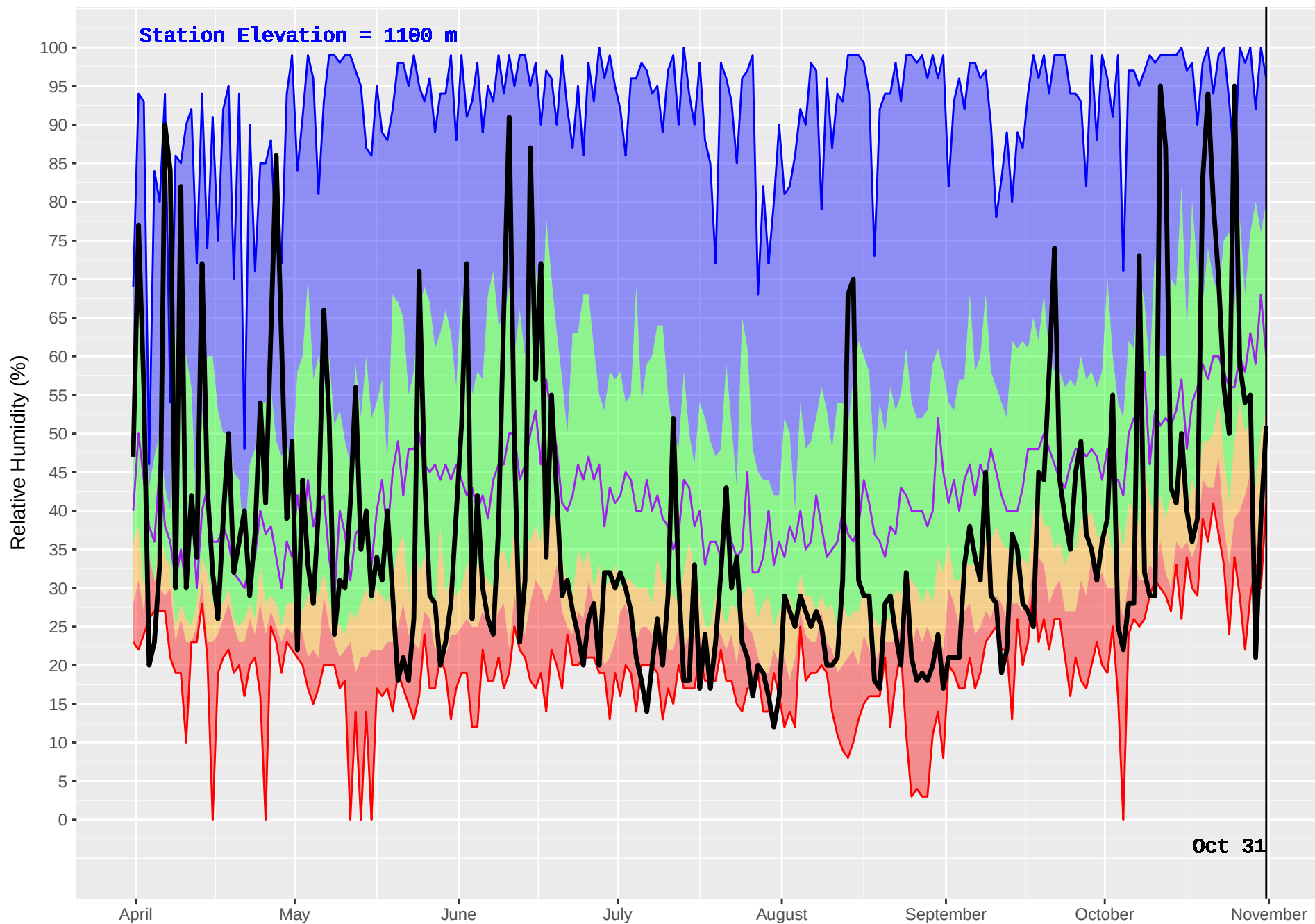
PALLISER (411) : Historical (1973–2016) and Current (2017) Noon Relative Humidity
