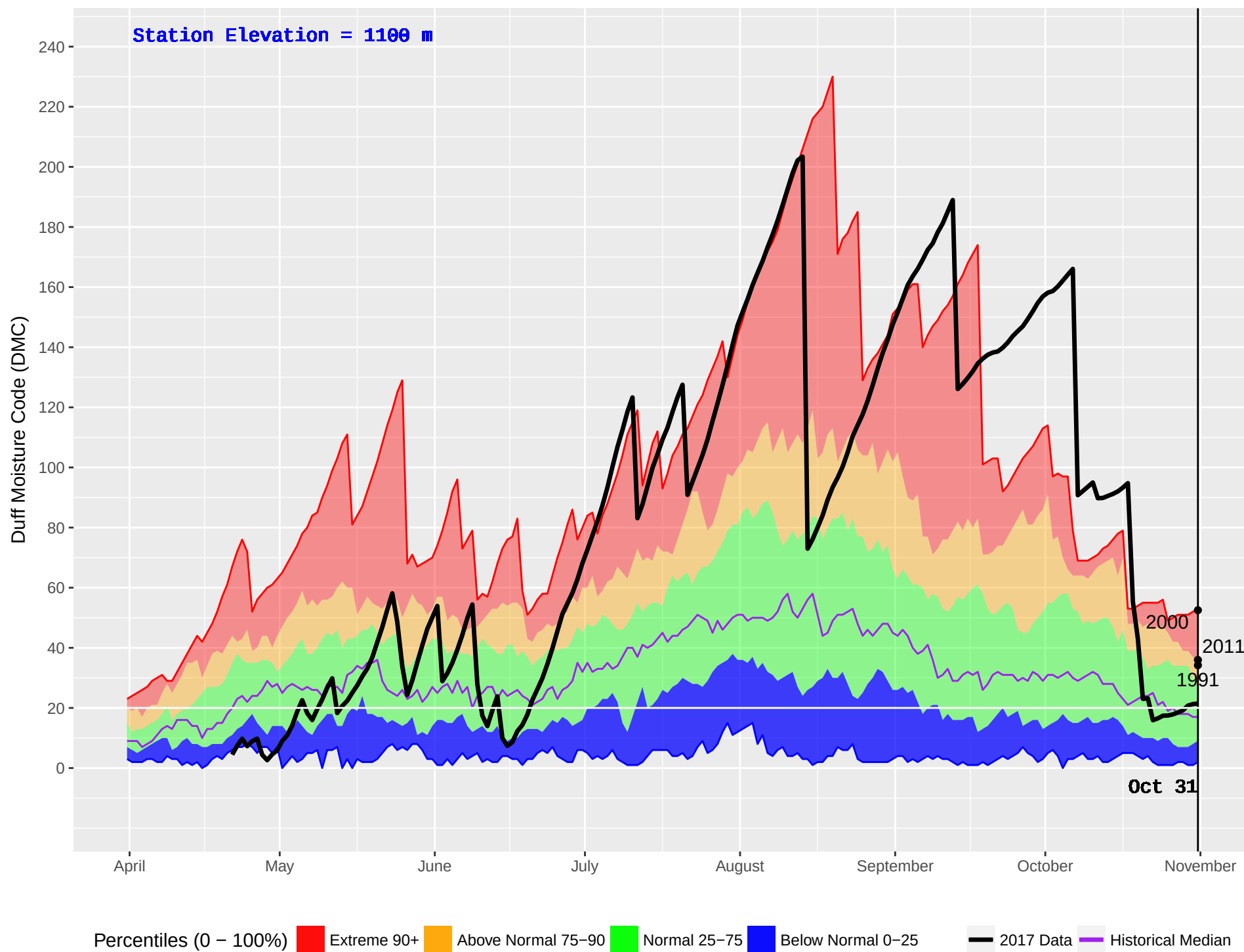
PALLISER (411) : Historical (1973–2016) and Current (2017) Noon Duff Moisture Code (DMC)
